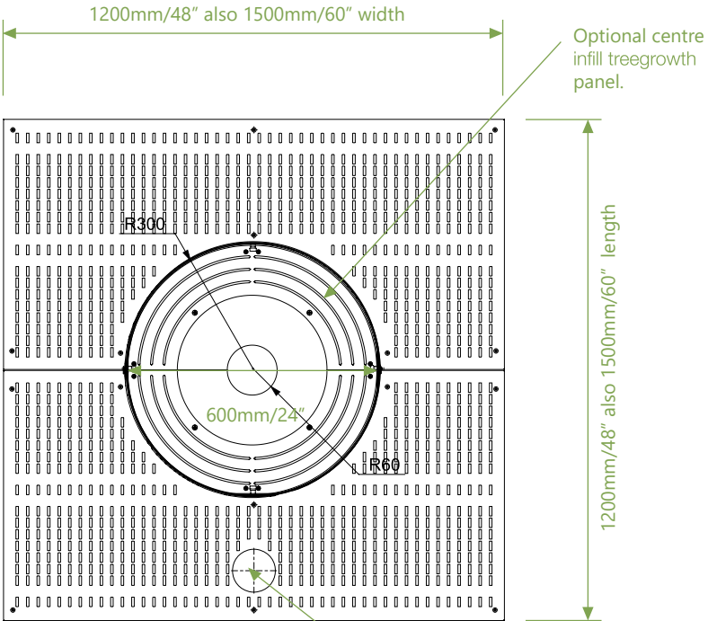
Plan View Optional Snorki™ inlet with hinged grate for watering and aeration.
